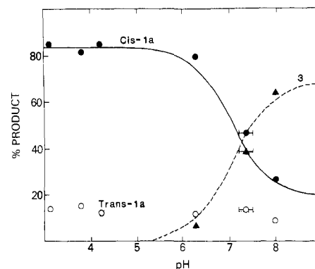
Figure 2. Dependence on pH of product distribution from the solvolysis of 1a in 10:90 (v/v) dioxane-water, ionic strength 0.1 M (NaClO 4 ) at 25 °C. The curves show the expected product distribution at intermediate pH values based on the distribution at high and low pH, assuming identical pH dependences for rate and product determination. The limiting product distribution at high pH was extrapolated from the observed value at pH 8.0 where ~90% of the reaction occurs via the k_0 pathway.
